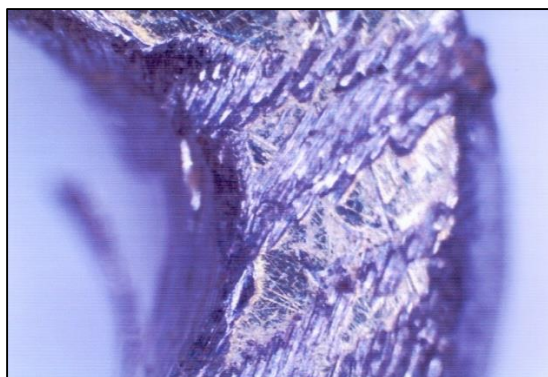
Fig. 4: Stereo microscopic images showing corrosion and metal release of titanium plates
